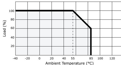
2. output power vs. ambient temperature (≥5 V)
