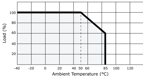
1. output power vs. ambient temperature (3.3 V)
